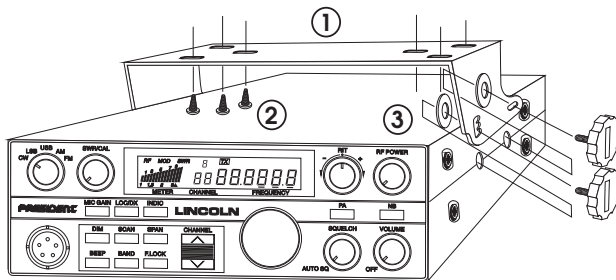
MOUNTING DIAGRAM
